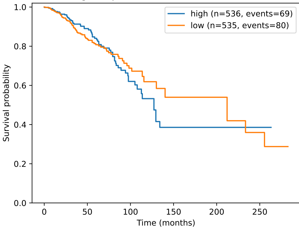
ESR1 — TCGA-BRCA logrank p=0.903 HR=1.02 (0.74-1.41)
